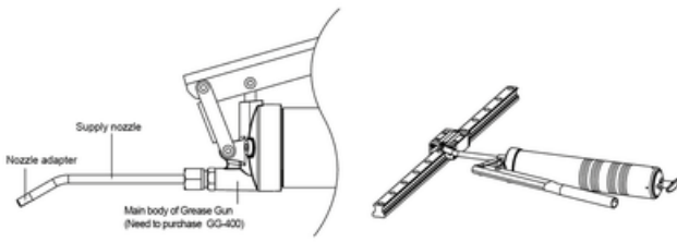
Nozzle adapter
